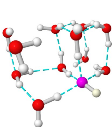
Figure 1. Computer model of an 11-water–OH - ion cluster. OH - is colored fuchsia. Hydrogen bonds are cyan.
